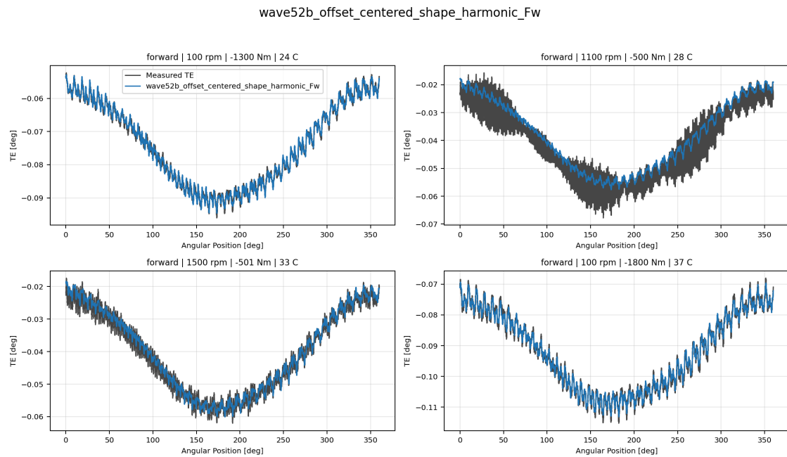
wave52b_offset_centered_shape_harmonic_Fw measured-versus-predicted TE collage
